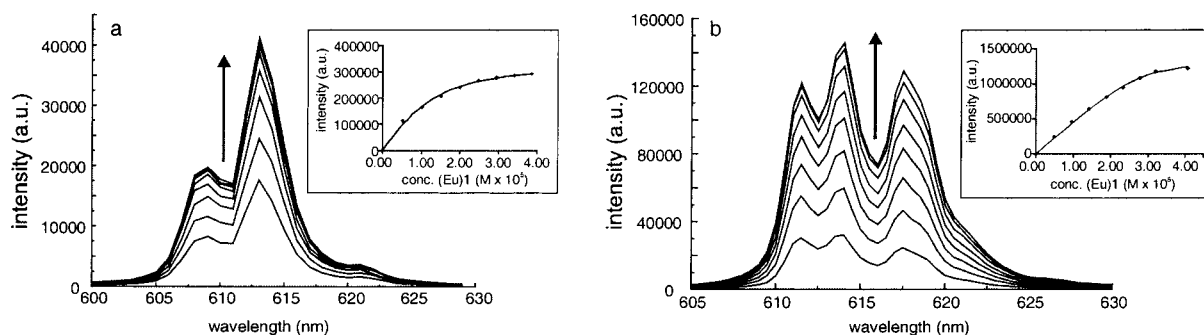
Figure 2. The increase in the sensitized {}^5D_0\text{--}{}^7F_2 emission band around 615 nm upon the addition of increasing concentrations of (Eu)1 to the aja (a) and bfa (b) antenna chromophores in dichloromethane. The insets show the formation of the ternary complexes as a function of the sensitized luminescence intensity. The solid lines are the theoretical curves for a 1:1 complex with K = 1.4 \pm 0.1 \times 10^5 \text{ M}^{-1} for [(Eu)1]aja and K = 3.8 \pm 0.2 \times 10^7 \text{ M}^{-1} for [(Eu)1]bfa, respectively.
