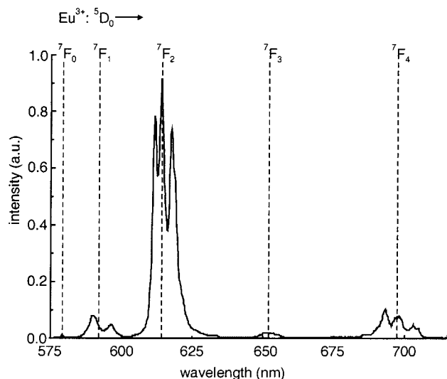
Figure 4. Magnification of the normalized emission spectrum ( \lambda_{\text{exc}} 330 nm) of [(Eu)1]bfa in dichloromethane ( 10^{-5} M). The emission bands have been assigned to the appropriate {}^5\text{D}_0\text{-}{}^7\text{F}_n transitions. The spectrum was recorded with a spectral bandwidth of 0.2 nm.
