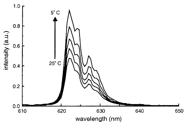
Figure 6. Increase of the luminescence intensity of [(Eu)I]dbm upon lowering the temperature from 25 °C to 5 °C.
